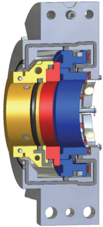
Split Seals
