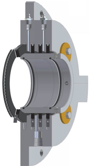
Split Bushing Seals
