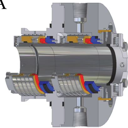
High Temperature Metal Bellows Seals
