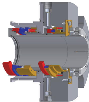
High Pressure Seals
