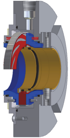
Non-contacting Seals
